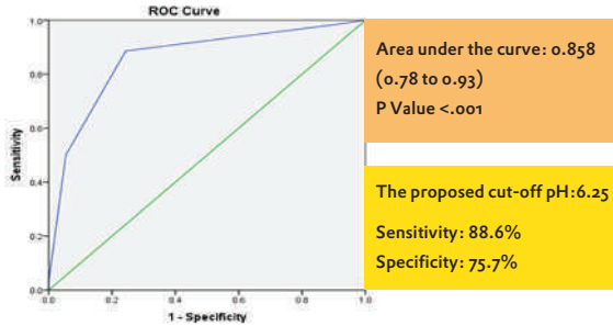
Fig 3 - ROC Analysis
